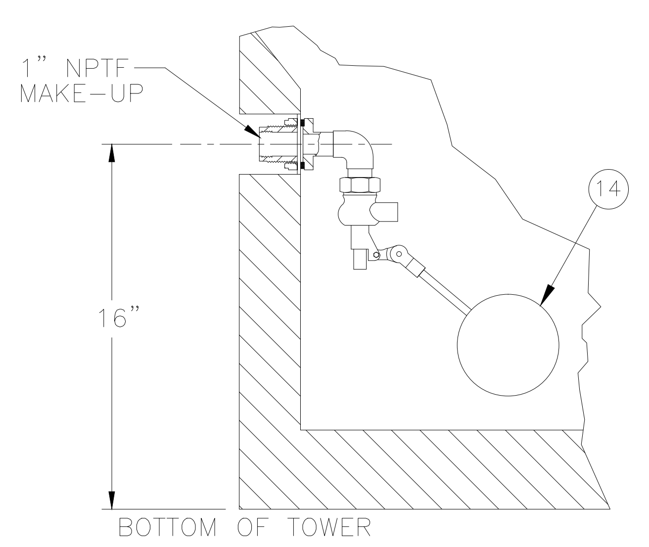
DETAIL A MAKE-UP NTS
