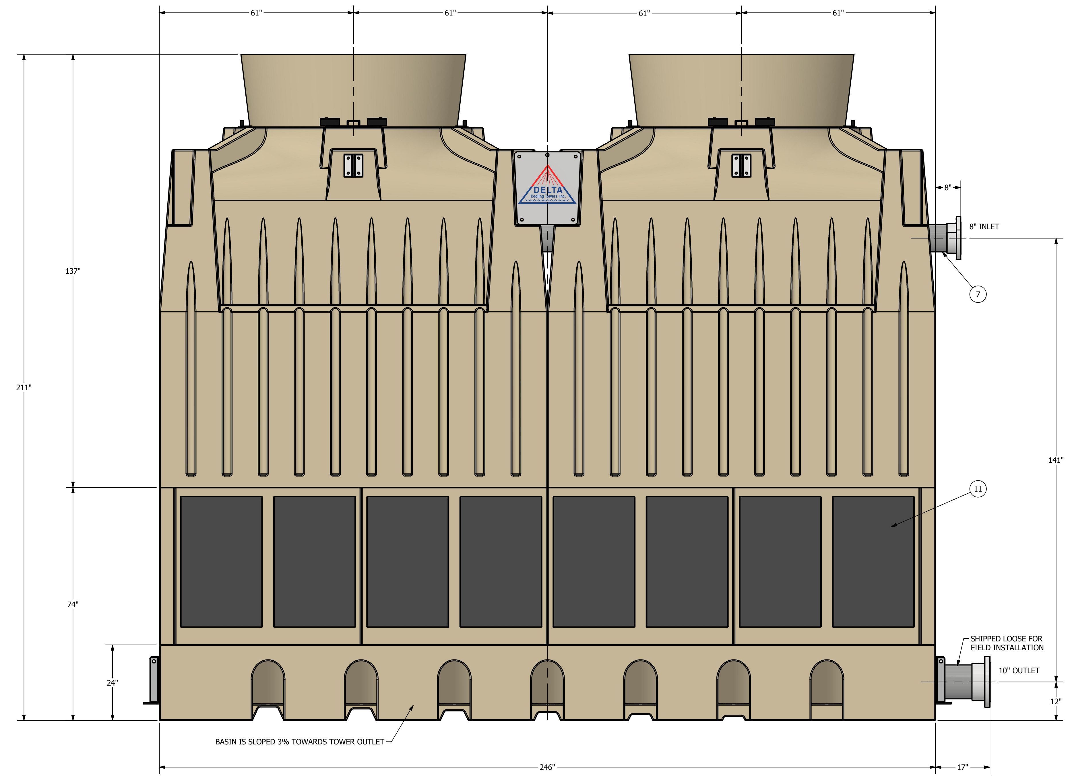
ELEVATION VIEW
