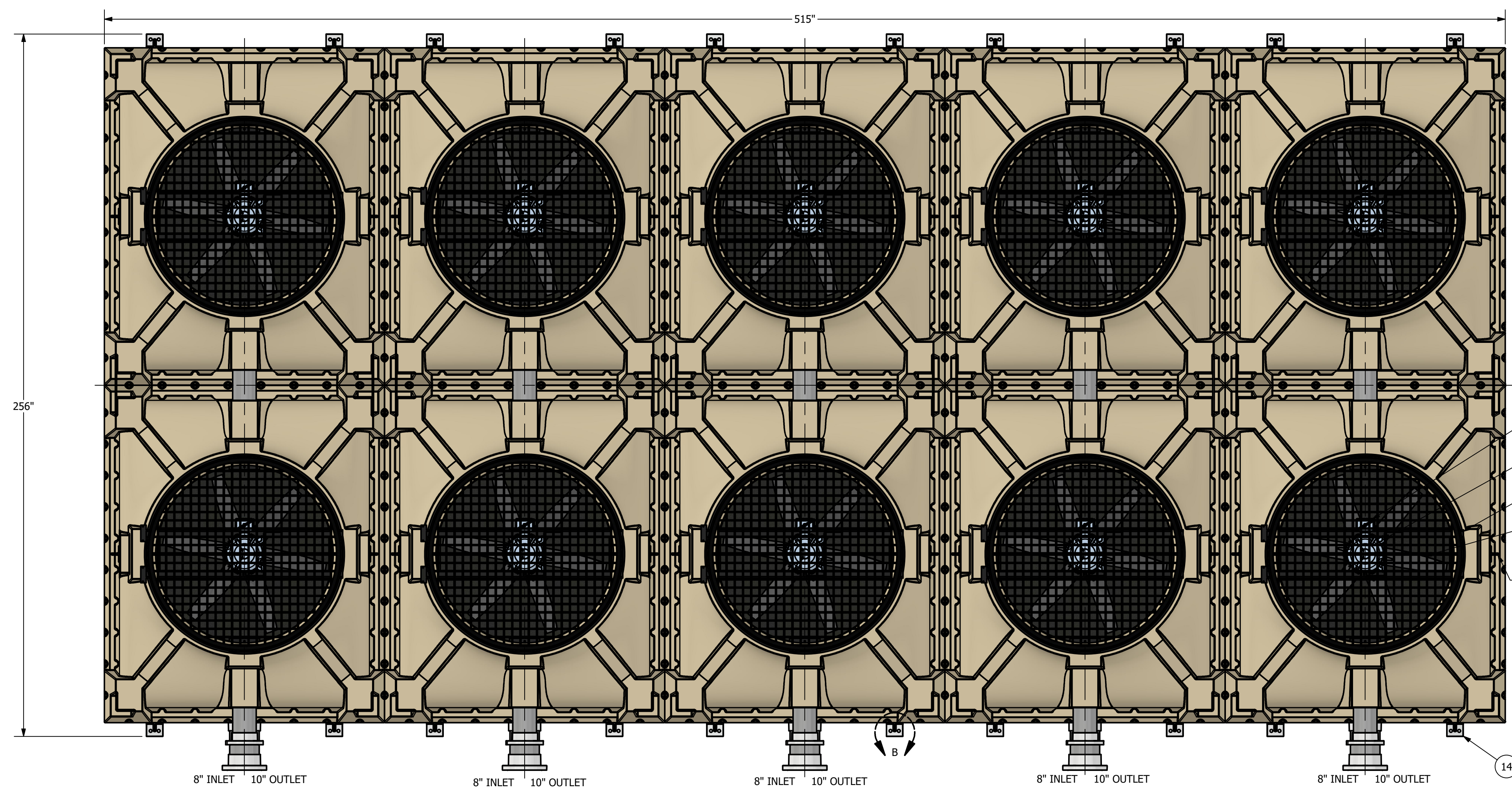
PLAN VIEW
