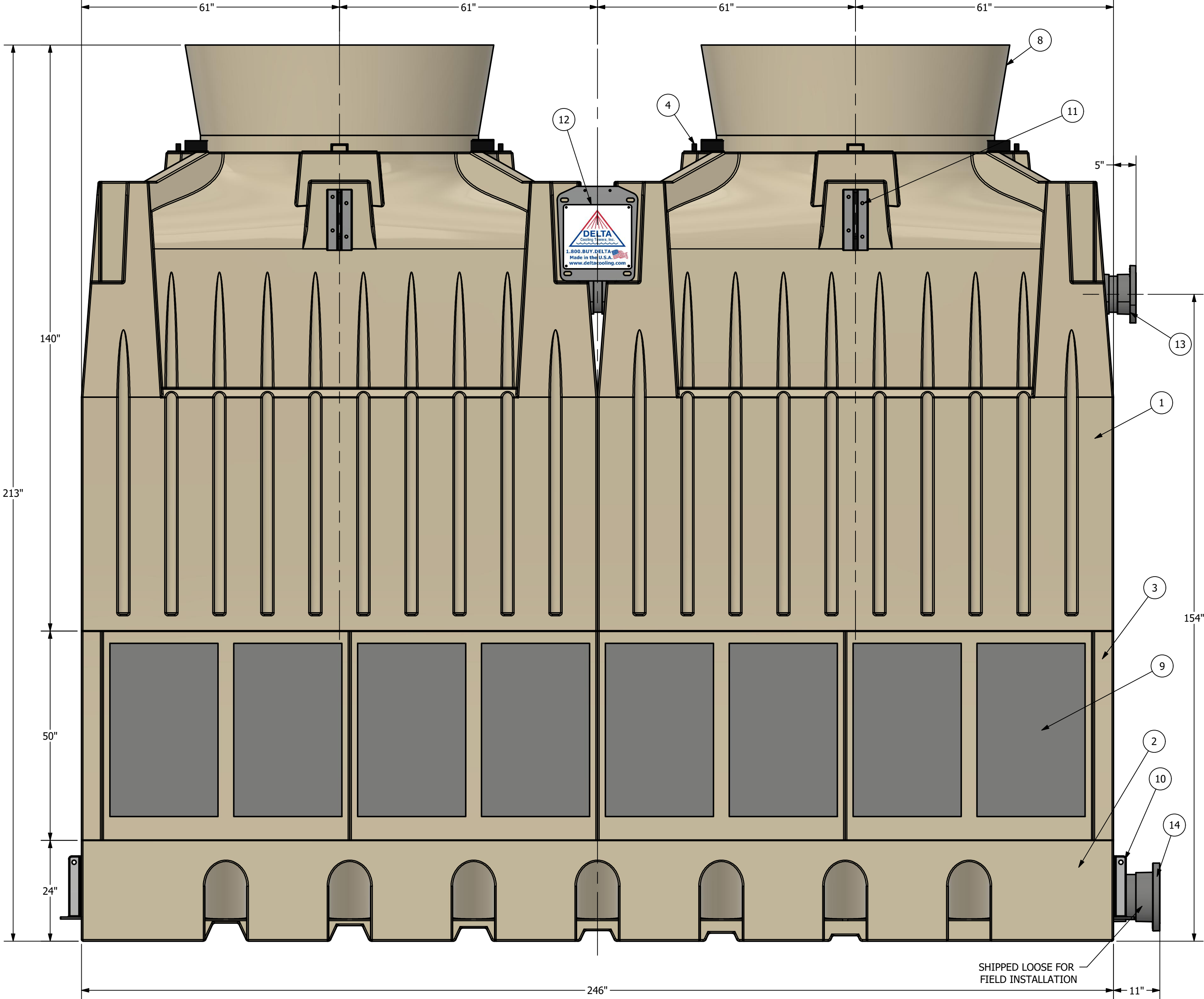
ELEVATION VIEW
